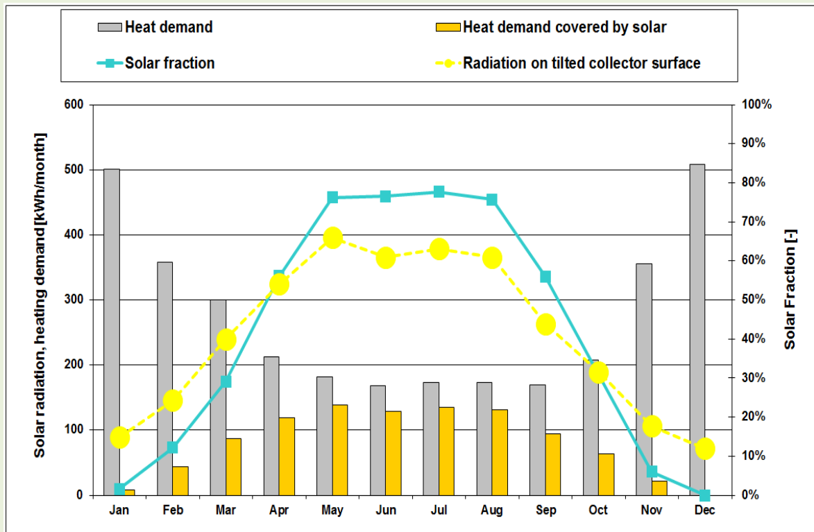
Figure 17: 3-bed Heat Demand and Solar Contribution (PHPP as designed – but re-implemented in PHPP8.5)
