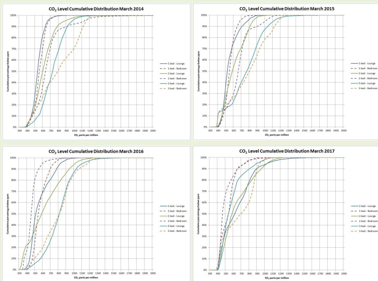
Figure 13: Distribution of Carbon Dioxide readings in March
